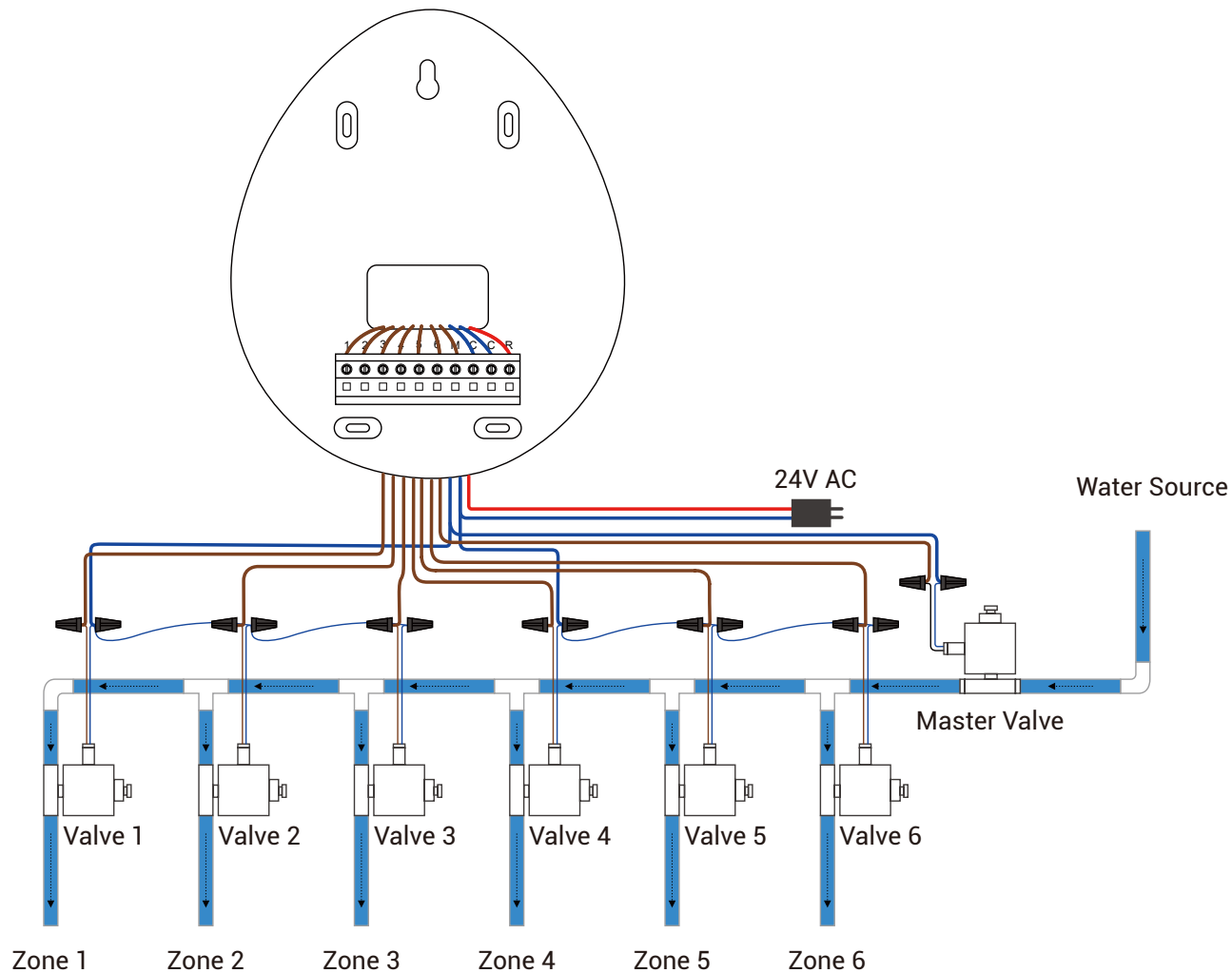
Wiring Diagram
